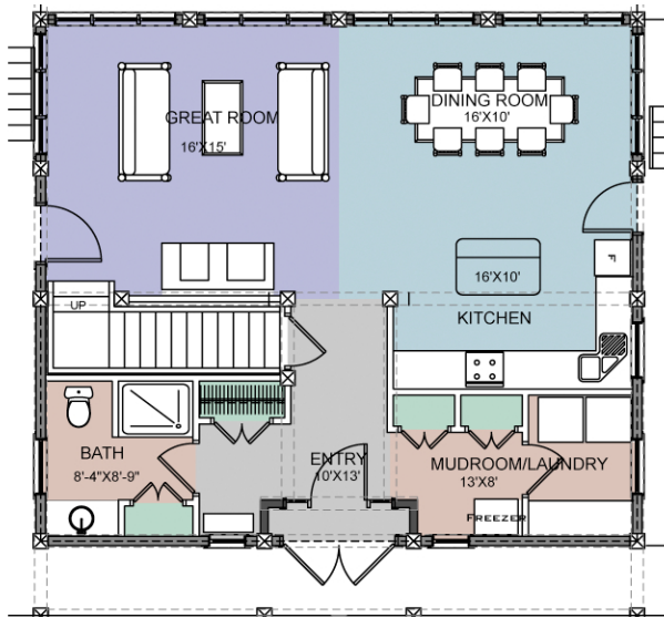
Main Level Floor Plan
